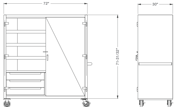
Spare Parts Cabinet Dimensions
